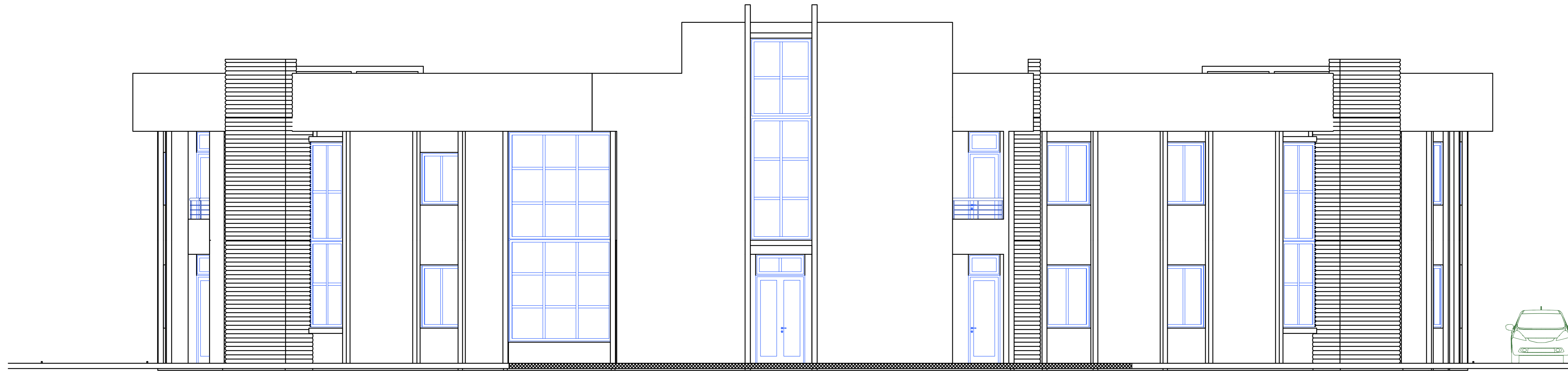
FACADE ARRIERE
